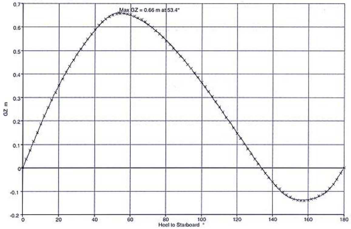
Elan 31 Gz Curve with Coachroof (standard Lead Keel)
