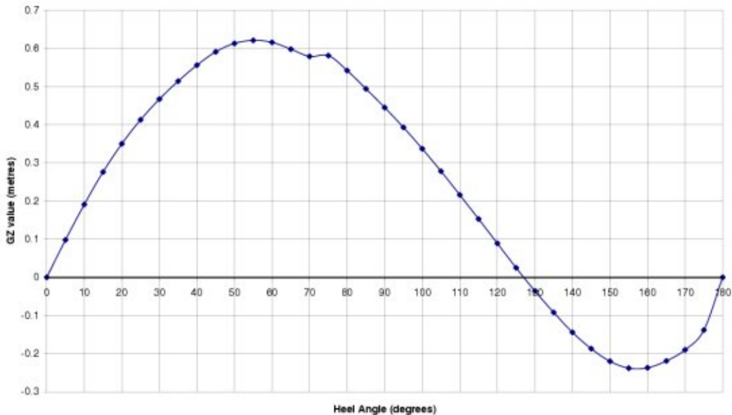
Elan 410 Preliminary GZ Curve
