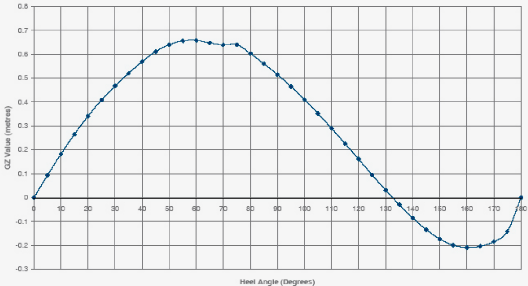
Elan 340 GZ Curve for the Composite Lead/Iron Performance Keel
